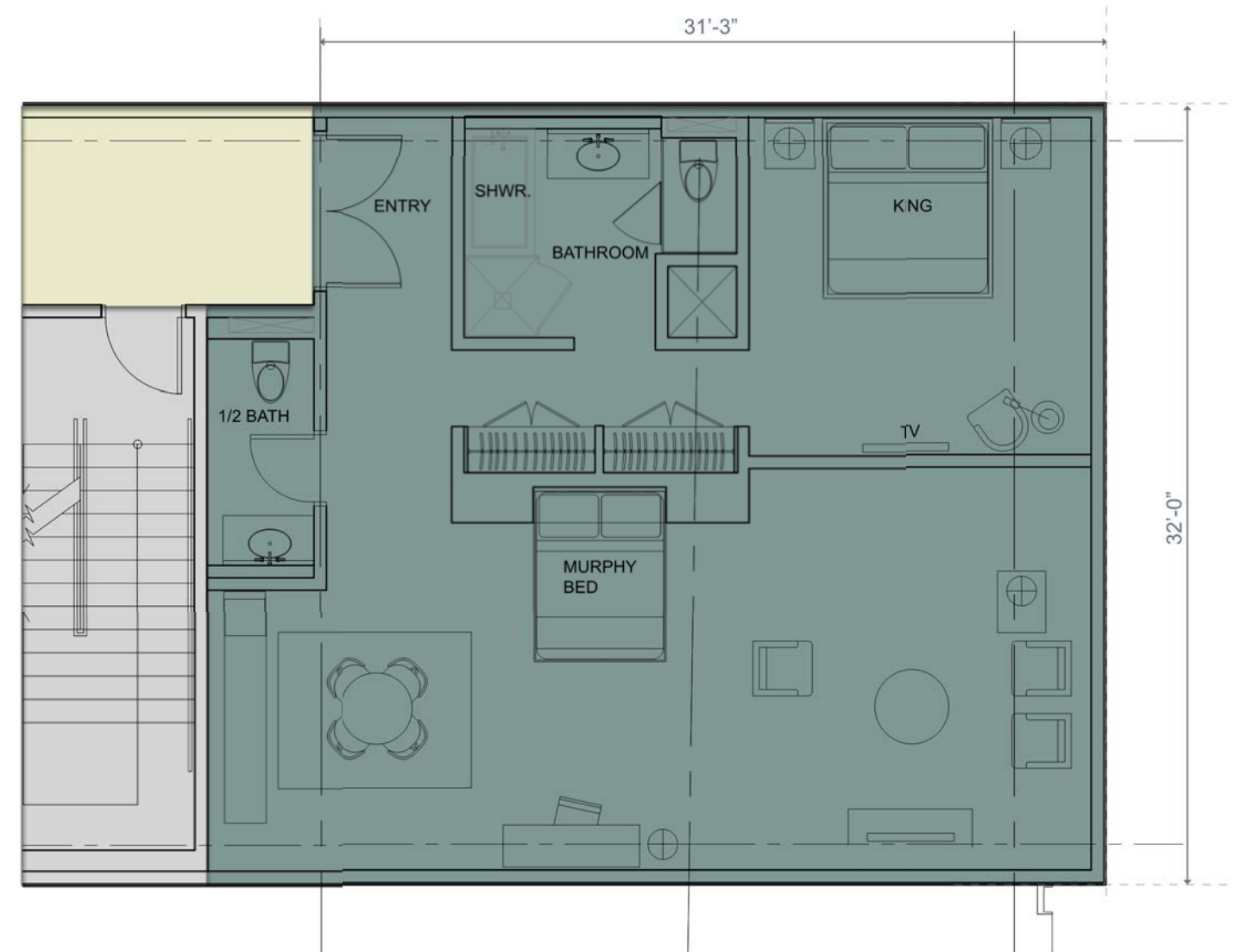
TYPICAL SUITE PLAN 1/2" = 1'-0"
