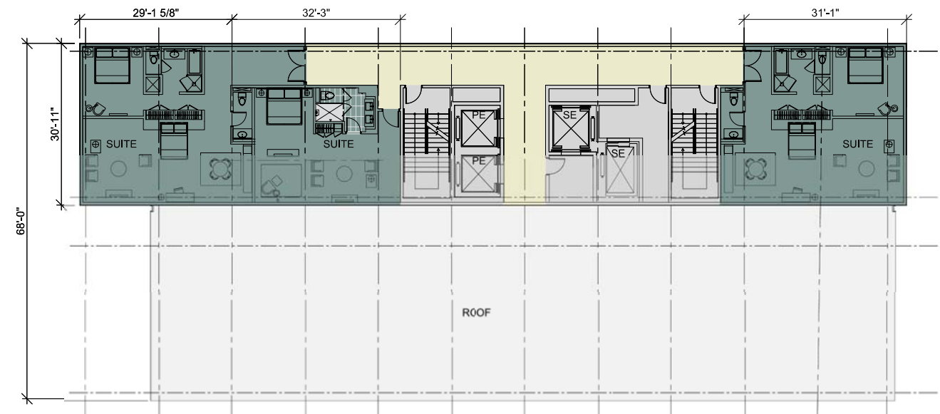
TYPICAL SUITE FLOOR PLAN
