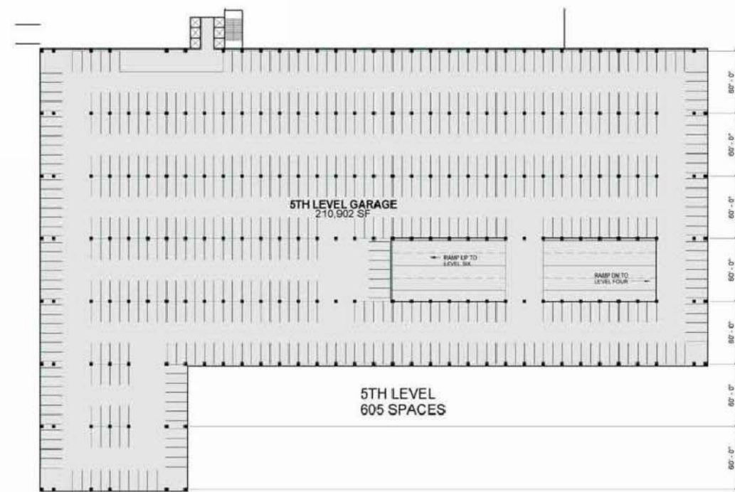
GARAGE A LVL 5 (@51' - 2") 1" = 40'-0"
