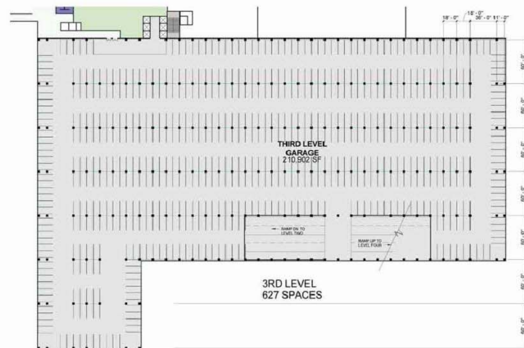
1F GARAGE A LVL 3 (@28' - 4") 1" = 40'-0"
