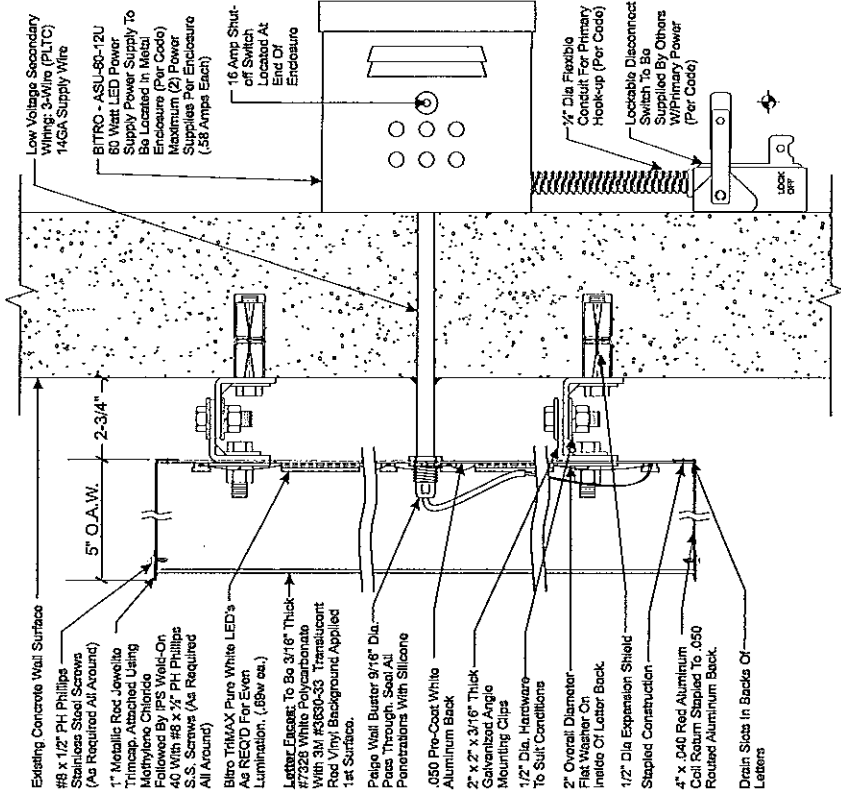
SECTION VIEW (TYPICAL) OF LETTERS SCALE: 3" = 1' 0"
