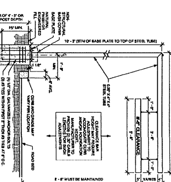
HIGH CLEARANCE BAR DETAIL
